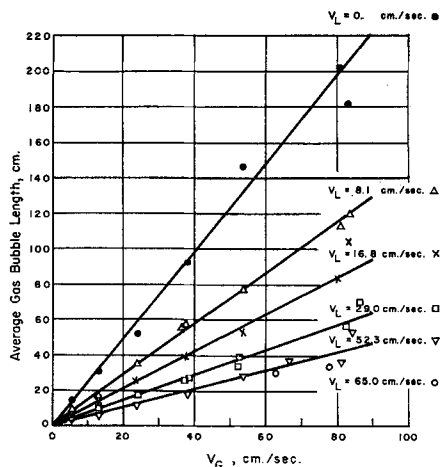
Fig. 7. Average gas bubble length vs. superficial gas velocity with superficial liquid velocity as parameter in a 1½-in. pipe at a 10 lb./sq.in. gauge inlet pressure.
