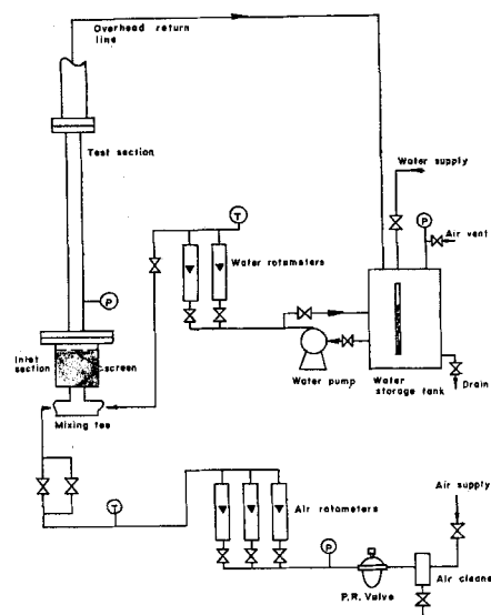
Fig. 2. Apparatus for the experimental investigation of gas-liquid slug flow.
