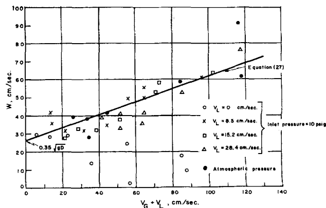
Fig. 5. The velocity of air bubbles through the surrounding water as a function of (v_g + v_L) in a 2\frac{1}{4} -in. I.D. pipe.
