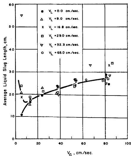
Fig. 6. Average liquid slug length vs. superficial gas velocity with superficial liquid velocity as parameter in a 1½-in. pipe at a 10 lb./sq.in. gauge inlet pressure.
